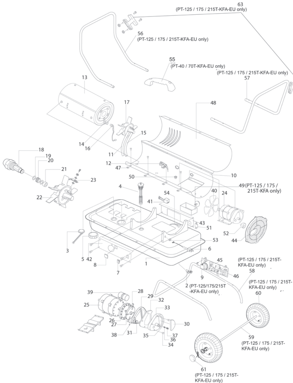
Figur 21: Delediagram for modeller PT-45/70T/125T/175T/215T-KFA-EU
