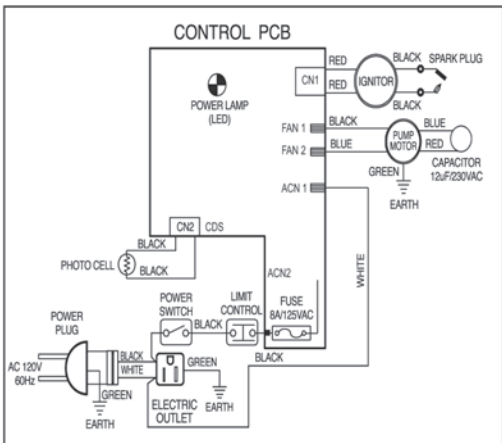
Figur 24: Modeller PT-125T/175T/215T-KFA-EU
